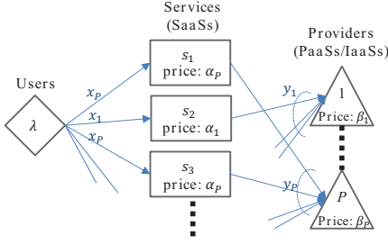
Figure 1: Overview of model structure and notation.
